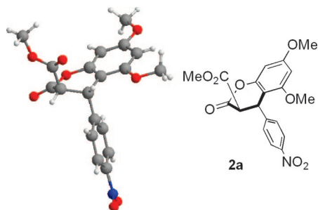
FIGURE 1. Crystal structure of 2a .
