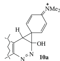
Figure 3. The assumed structure of cation 10a .
