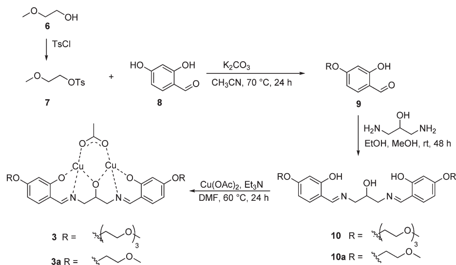
Scheme 2. Synthesis of Schiff Base Complex 3a
