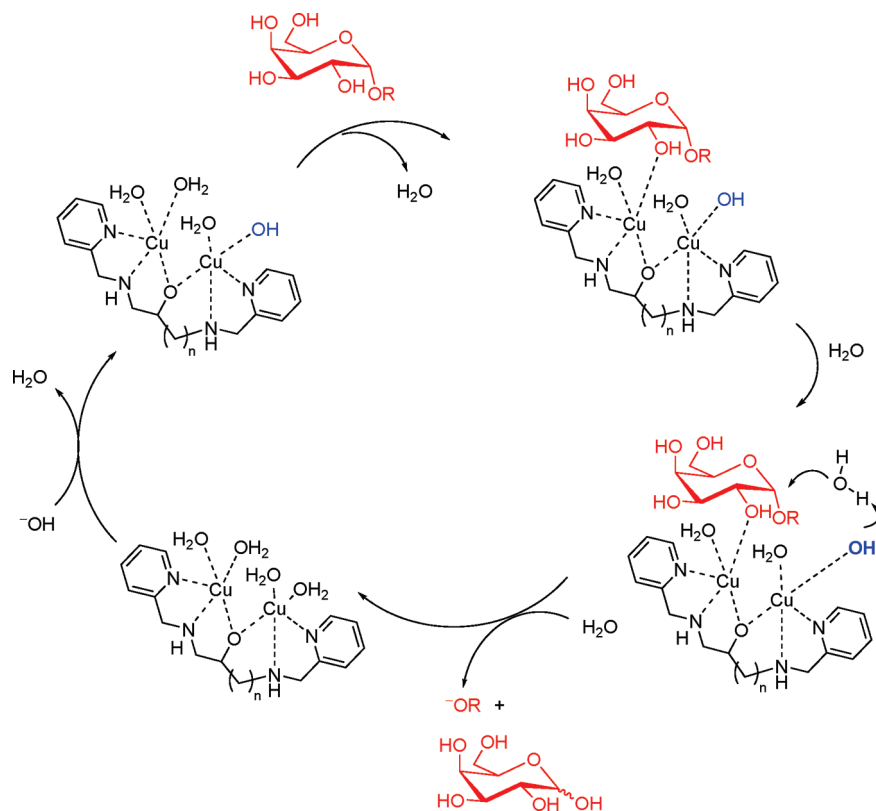
Scheme 6. Putative Mechanism for the Hydrolysis of 12 by 1 ( n = 1 ) or 2 ( n = 2 ) a
