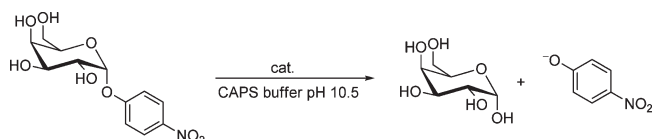
Scheme 5. Catalytic Hydrolysis of p -Nitrophenyl- \alpha -D-galactopyranoside ( 12 )
