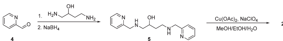
Scheme 1. Synthesis of Asymmetric Complex 2
