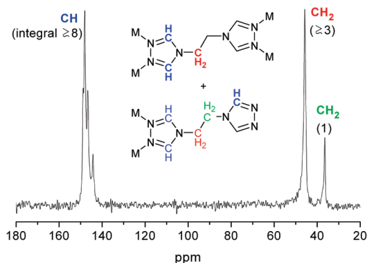
Figure 23. ^{13}\text{C} CPMAS NMR spectrum for 8 (example also for 9 ) and schematic drawing of the building unit with the unique C atoms as atom symbols. All atoms of the \mu_2 - \kappa\text{N}1:N2 -bridging, dangling btre ligand have half-occupancy (indicated by plain font style). Integral of \text{CH}_2 resonance around 37 ppm set to 1. Peak positions: 148.8, 148.1, 146.6, 144.2, 45.7, and 36.5 ppm (148.4, 147.6, 146.3, 144.3, 45.6, and 37.2 ppm for 9 , cf. Figure S27, Supporting Information).
