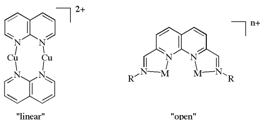
Figure 1. Representations of known and possible types of naphthyridine complex.
