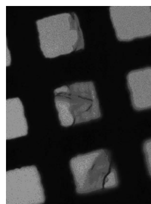
Figure 12. DIC image ( \times 40 ) of a cross-linked monolayer of 16a taken 5 days after the transfer event. The film is on a Cu grid with 2025\text{ }\mu\text{m}^2 -sized holes, some of which are spanned over by non-ruptured films (holes on the right-hand side) and others are not at all (holes on the left-hand side). The holes in the center are partially covered by films and overlapping parts, wrinkles, and rolled-up edges are visible.
