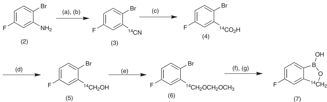
Scheme 1 Conditions: (a) 1 M H 2 SO 4 , 4 M HCl, NaNO 2 , water, 4°C; (b) Cu 14 CN, K 14 CN, water 0°C; (c) H 2 SO 4 , 140°C; (d) BH 3 –THF, THF; (e) ClCH 2 OCH 3 , ( i -Pr) 2 NEt, CH 2 Cl 2 ; (f) n -BuLi, THF, B(O- i -Pr) 3 , –78°C to room temperature; and (g) 6 N HCl.
