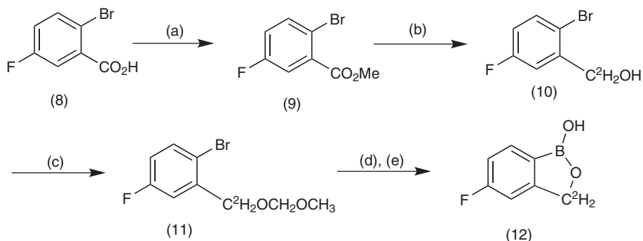
Scheme 2 Conditions: (a) MeOH, H 2 SO 4 , room temperature for 2 days then reflux for 1 day; (b) LiEt 3 B 2 H, THF 0°C, 16 h; (c) ClCH 2 OCH 3 , ( i -Pr) 2 NEt, CH 2 Cl 2 ; (d) t -BuLi, THF, B(OMe) 3 , –78°C to room temperature; and (e) 6 N HCl.
