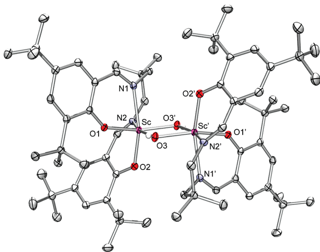
Figure 4. Solid-state structure of complex [(\text{Salpren})\text{Sc}(\mu\text{-OH})_2] ( 3b ). Heavy atoms are represented by atomic displacement ellipsoids at the 50% level. Hydrogen atoms, except for H1OH and H1OH', and cocrystallized \text{C}_6\text{D}_6 are omitted for clarity.
