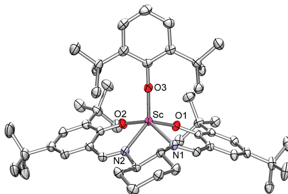
Figure 6. Solid-state structure of complex (\text{Salcyc})\text{Sc}(\text{OAr}^{\text{tBu},\text{tBu}}) ( 4b ). Heavy atoms are represented by atomic displacement ellipsoids at the 50% level. Hydrogen atoms are omitted for clarity.
