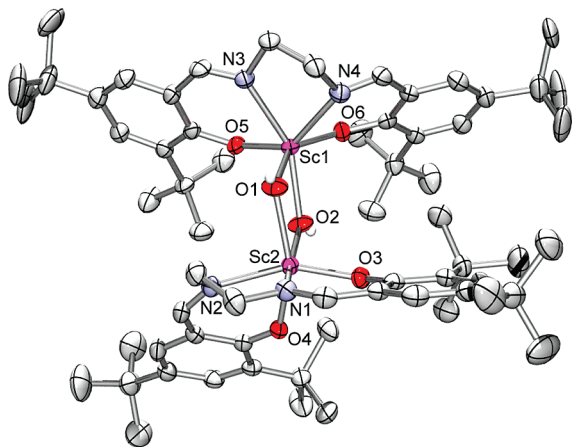
Figure 3. Solid-state structure of complex [(\text{Salen})\text{Sc}(\mu\text{-OH})_2] ( 3a ). Heavy atoms are represented by atomic displacement ellipsoids at the 50% level. Hydrogen atoms, except for H1O and H2O, and cocrystallized toluene are omitted for clarity.
