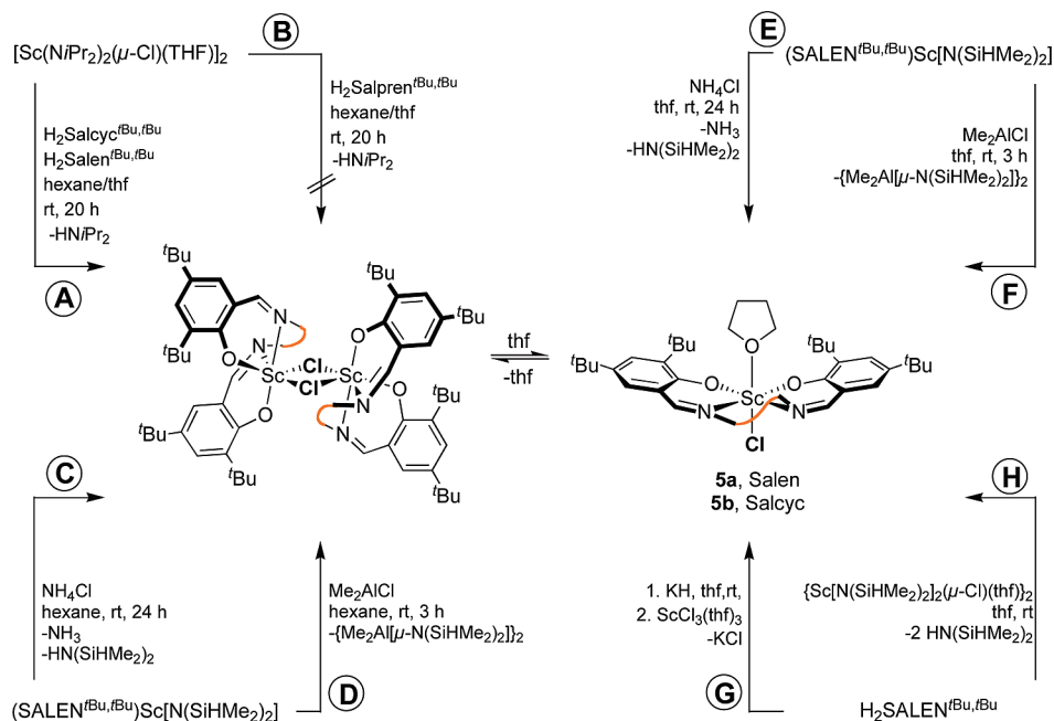
Scheme 3. Different Synthesis Protocols for Dimeric and Monomeric Sc–SALEN Chloride Complexes a
