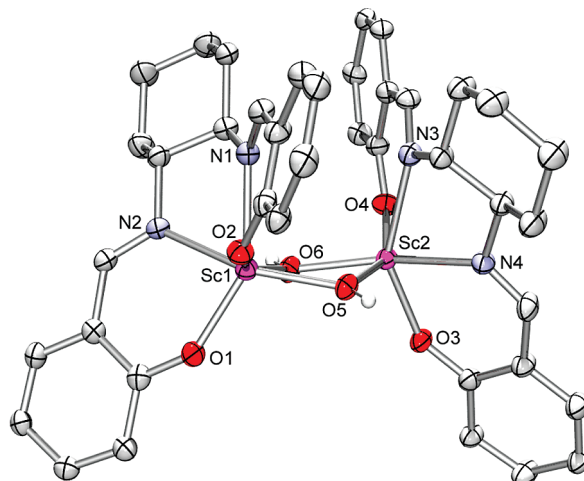
Figure 5. Solid-state structure of complex [(\text{Salcyc})\text{Sc}(\mu\text{-OH})_2] ( 3c ). Heavy atoms are represented by atomic displacement ellipsoids at the 50% level. Hydrogen atoms, except for H5O and H6O, t Bu-substitution in the 3- and 5- positions, and cocrystallized toluene are omitted for clarity.
