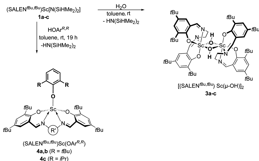
Scheme 2. High-Yield Protonolysis Reactions of (\text{SALEN}^{\text{tBu,tBu}}\text{Sc}[\text{N}(\text{SiHMe}_2)_2]) ( 1a–c ) with \text{HOAr}^{\text{tBu,tBu}} , \text{HOAr}^{\text{tPr,tPr}} , and \text{H}_2\text{O}
