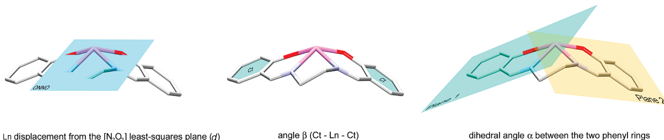
Figure 1. Coordination features of SALEN ligands.
