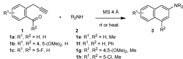
Scheme 1. Synthesis of 2-Aminonaphthalene Derivatives via Aminobenzannulation without Metallic Catalysts
