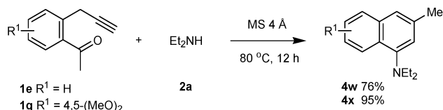
Scheme 3. Formation of 1-Aminonaphthalene Derivatives
