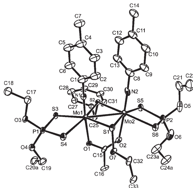
Figure 2. ORTEP view of the cation \text{BnS}\{\text{Mo}_2\}\text{SOEt}^+ , 4^+(\text{Et}) .
