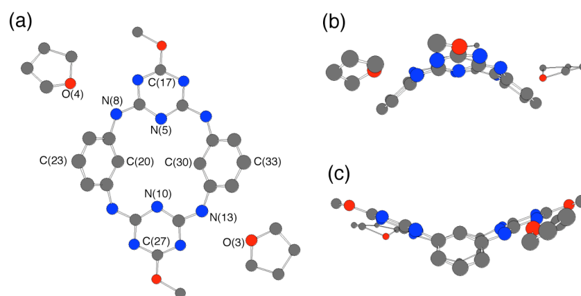
Figure 2. Crystal structure of 4 ·2THF: top view (a) and side views (b and c). Hydrogen atoms are excluded for clarity.
