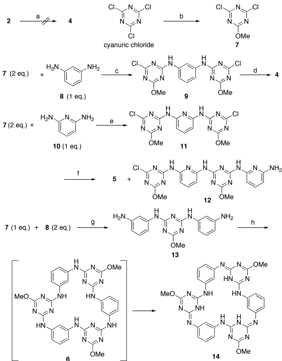
Scheme 1. Synthesis of aza-calix(4-methoxy)triazines 4-6 . (a) MeOH, i Pr 2 NEt, reflux; (b) MeOH, NaHCO 3 , H 2 O, 0 °C, 2.5 h, 98%; (c) i Pr 2 NEt, THF, rt, 50 min, 98%; (d) 8 , i Pr 2 NEt, THF, 100 °C, 72 h, 68%; (e) i Pr 2 NEt, THF, rt, 48 h, 65%; (f) 10 , i Pr 2 NEt, THF, 130 °C, 120 h, (g) i Pr 2 NEt, THF, 60 °C, 48 h, 55%; (h) 9 , i Pr 2 NEt, THF, 100 °C, 72 h, 57%.
