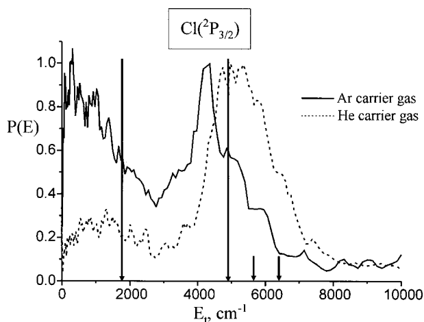
FIG. 5. \text{Cl}(^2P_{3/2}) signals obtained following 266 nm dissociation of \text{CH}_2\text{Cl} ( 37\,594 \text{ cm}^{-1} ) using Ar (solid line) or He (dotted line) carrier gas plotted as a function of the total c.m. photofragment translational energy, E_t . The long arrows indicate the energy thresholds for the production of \text{CH}_2(\tilde{X}^3B_1) and \text{CH}_2(\tilde{a}^1A_1) from vibrationally “cold” \text{CH}_2\text{Cl} (see Fig. 2). The short arrows show the positions of “hot band” peaks which are resolved in the Ar experiments.
