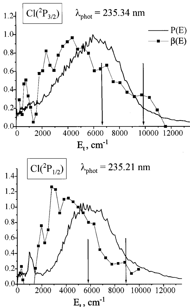
FIG. 7. Total c.m. translational energy (solid lines) and angular anisotropy parameter (squares) distributions of \text{Cl}(^2P_{3/2}) (upper panel) and \text{Cl}(^2P_{1/2}) (lower panel) obtained in one-color experiments at 235.34 nm and 235.21 nm, respectively. Arrows show the energy thresholds for production of \text{CH}_2(\tilde{X}^3B_1) and \text{CH}_2(\tilde{a}^1A_1) .
