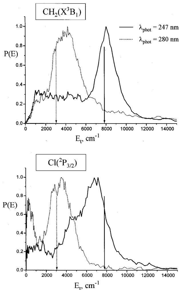
FIG. 3. CH 2 ( \tilde{X}^3B_1 ) (top panel) and Cl( ^2P_{3/2} ) (bottom panel) signals obtained following 247 nm (40 486 cm -1 ; solid lines) and 280 nm (35 714 cm -1 ; dotted lines) dissociation of CH 2 Cl plotted as a function of the total c.m. photofragment translational energy, E_t , as described in Fig. 2. The arrows indicate the energy thresholds calculated using D_0=391 kJ/mol.
