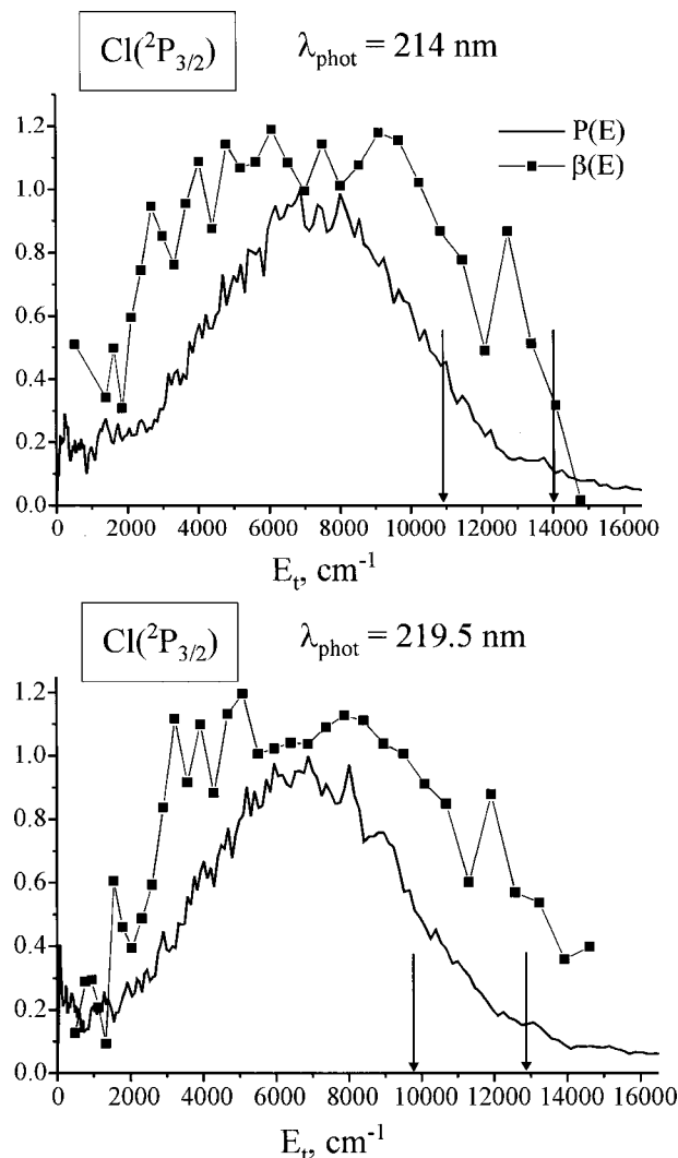
FIG. 8. Total c.m. translational energy (solid lines) and angular anisotropy parameter (squares) distributions of \text{Cl}(^2P_{3/2}) obtained from the dissociation of \text{CH}_2\text{Cl} at 214 nm (upper panel) and 219.5 nm (lower panel) and detected by (2+1) REMPI at 235.34 nm. Arrows show the energy thresholds for production of \text{CH}_2(\tilde{X}^3B_1) and \text{CH}_2(\tilde{a}^1A_1) .
