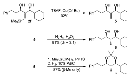
Scheme 3. Reduction of syn -1,3-Diol 2f
