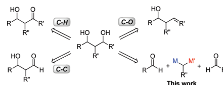
Figure 1. Synthesis of 1,3-diols.
