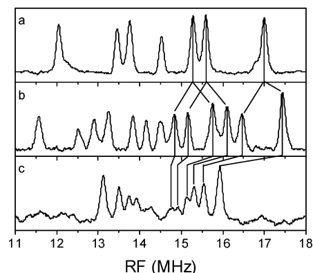
Figure 6. 1 H ENDOR spectra of 1a •− (a), 1c •− (b), and 2a •− (c) in DMF with ~1–4% TEA (w/w) at 290 K. Microwave powers were 2–20 mW, and RF power was 240–400 W with a frequency modulation depth of 100 kHz.
