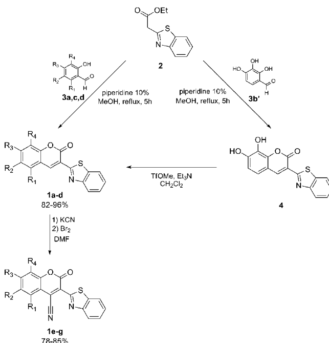
Scheme 2. Synthesis of Coumarins; Substituents: R 1 = R 4 = H, R 2 = R 3 = OMe ( a , e ); R 1 = R 2 = H, R 3 = R 4 = OMe ( b , f ); R 1 = R 2 = H, R 3 , R 4 = –O–CH 2 –CH(COOEt)–O– ( c , g ); R 1 , R 2 = fused phenyl ring, R 3 = R 4 = H ( d ); R 1 = R 2 = H, R 3 = R 4 = OH ( 4 )
