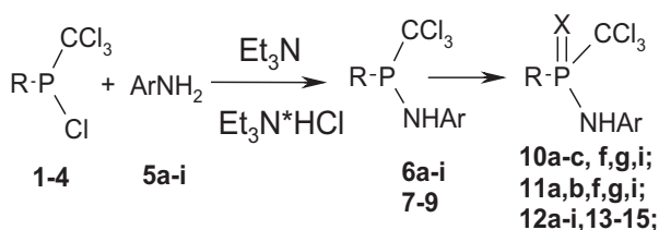
Scheme 2. Synthesis of the starting materials 10–15 .
