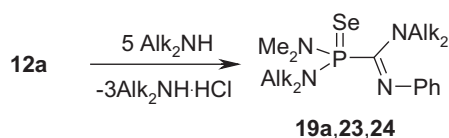
Scheme 5. Influence of amines.
