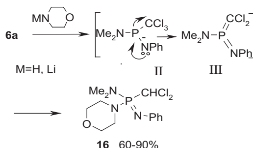
Scheme 3. Reaction of P(III) compounds with amines.
