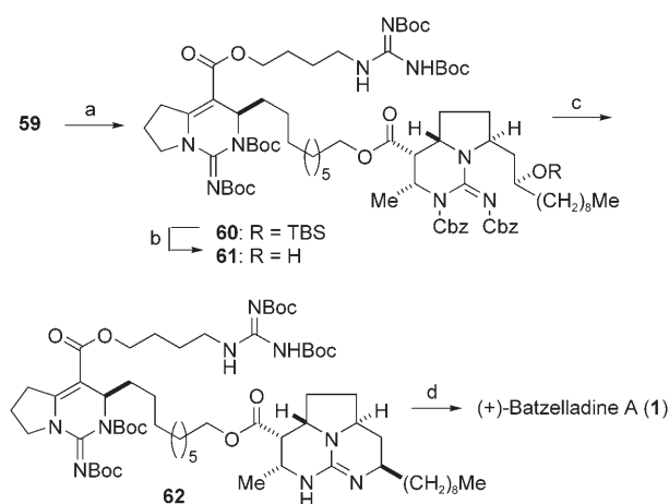
Scheme 12. Total synthesis of (+)-batzelladine A (1) . Reagents and conditions: a) 35 , \text{EDCl} , DMAP, \text{CH}_2\text{Cl}_2 , 0^\circ\text{C} , 60%; b) \text{HF}/\text{pyridine} , THF, 0^\circ\text{C} , 89%; c) 1) \text{Pd/C} , \text{H}_2 , \text{EtOAc} , RT; 2) \text{DEAD} , \text{PPh}_3 , toluene, RT; d) \text{TFA}/\text{CH}_2\text{Cl}_2 , RT, 24% (from 61 ).
