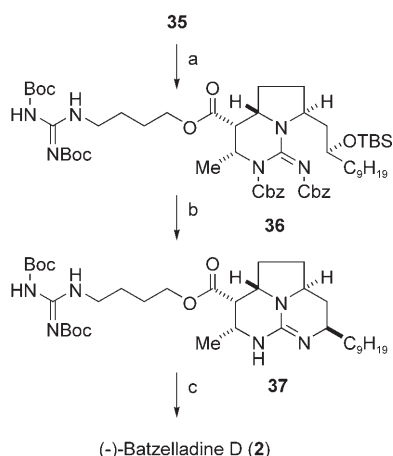
Scheme 6. Total synthesis of (–)-batzelladine D ( 2 ). Reagents and conditions: a) 8 , EDCI, DMAP, \text{CH}_2\text{Cl}_2 , 0°C, 66% (from 34 ); b) 1) HF/pyridine, THF, 0°C, 81%; 2) Pd/C, \text{H}_2 , EtOH, RT; 3) DEAD, \text{PPh}_3 , toluene, RT; c) TFA, \text{CH}_2\text{Cl}_2 , RT, 66% (3 steps).
