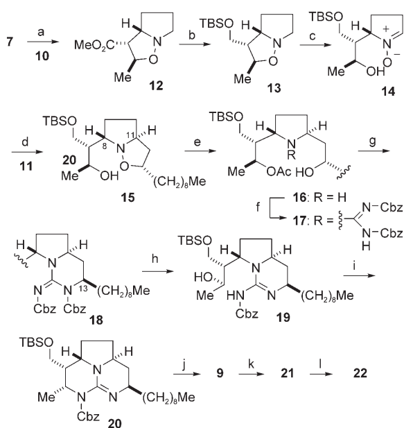
Scheme 3. Synthesis of the tricyclic guanidine carboxylic acid 9 . Reagents and conditions: a) methyl crotonate ( 10 ), toluene, 100°C, 82%; b) 1) LiAlH 4 , Et 2 O, 0°C; 2) TBSO, imidazole, CH 2 Cl 2 , RT, 95% (2 steps); c) mCPBA, CH 2 Cl 2 , 0°C; d) 1-undecene ( 11 ), toluene, 110°C, 76% (2 steps); e) 1) Ac 2 O, pyridine, RT; 2) Pd/C, H 2 , EtOH, RT, 98% (2 steps); f) bis-Cbz-2-methyl-2-thiopseudourea, HgCl 2 , Et 3 N, DMF, 0°C to RT, 52%; g) DEAD, PPh 3 , THF, RT, 58%; h) NaH, THF/MeOH (1:1), RT, 80%; i) MsCl, Et 3 N, CH 2 Cl 2 , 0°C, 82%; j) Jones reagent, acetone, 0°C; k) TMSCHN 2 , PhH/MeOH (7:2), RT, 47% (2 steps); l) Pd/C, H 2 , EtOH, RT, 85%.
