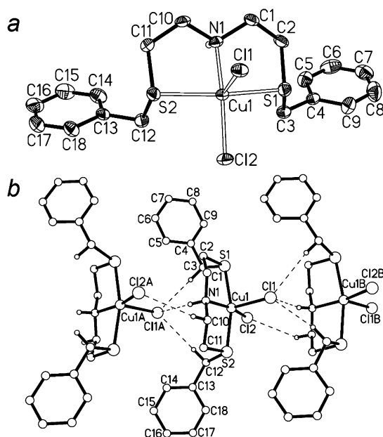
Figure 2. (a) Thermal ellipsoids at 30% probability of the molecular structure of 1 . Selected bond distances [Å] and angles [deg]: Cu1–N1 2.001(4), Cu1–S1 2.353(1), Cu1–S2 2.380(1), Cu1–Cl2 2.241(1), Cu1–Cl1 2.518(1), N1–Cu1–Cl2 162.4(1), N1–Cu1–S1 85.4(1), N1–Cu1–S2 85.3(1), N1–Cu1–Cl1 92.3(1), S1–Cu1–S2 165.44(5), S1–Cu1–Cl1 94.39(4), S2–Cu1–Cl1 97.07(4), Cl2–Cu1–Cl1 105.29(5), Cl2–Cu1–S1 92.84(5), Cl2–Cu1–S2 92.76(5). (b) A crystal structure representation showing secondary intermolecular H bonding in 1 . (Cu1...Cu1A 5.829 Å, symmetry code A: x, 1.5 - y, -0.5 + z ).
