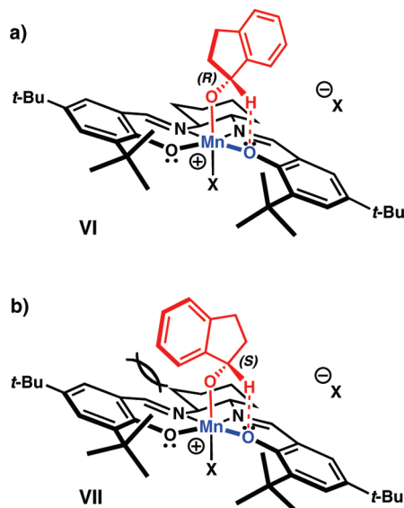
Figure 3. Plausible pre-transition-state assemblies for the (a) favored and (b) disfavored modes of oxidation.
