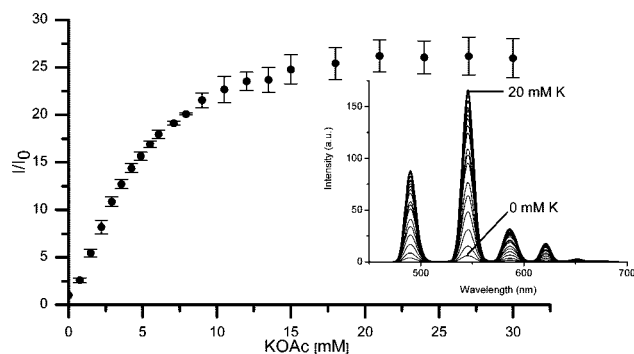
Figure 2. Relative time delayed luminescence of Tb-1 as a function of K^+ concentration (error bars represent standard deviation (s.d.), n = 3 ). Inset, luminescence spectra of Tb-1• K^+ titration. Excitation at 332 nm, emission at 545 nm, time delay 0.2 ms, [Tb-1] = 50 \mu M , T = 20^\circ C .
