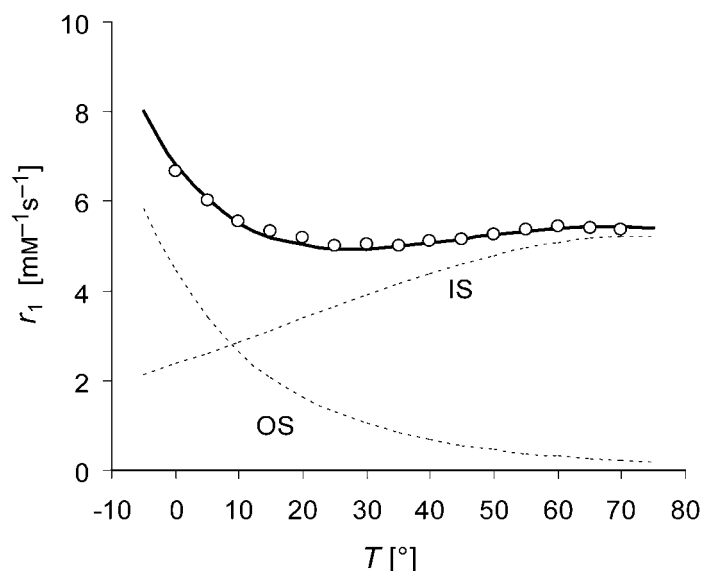
Fig. 2. Temperature dependence of the 20-MHz relaxivity of [Gd^{III}(8)]^{3-} in aqueous solution at pH 7.0. The solid line reflects the best fit of the data to the SBM theory, the dotted lines show the individual outer-sphere (OS) and inner-sphere (IS) contributions [27][36].
