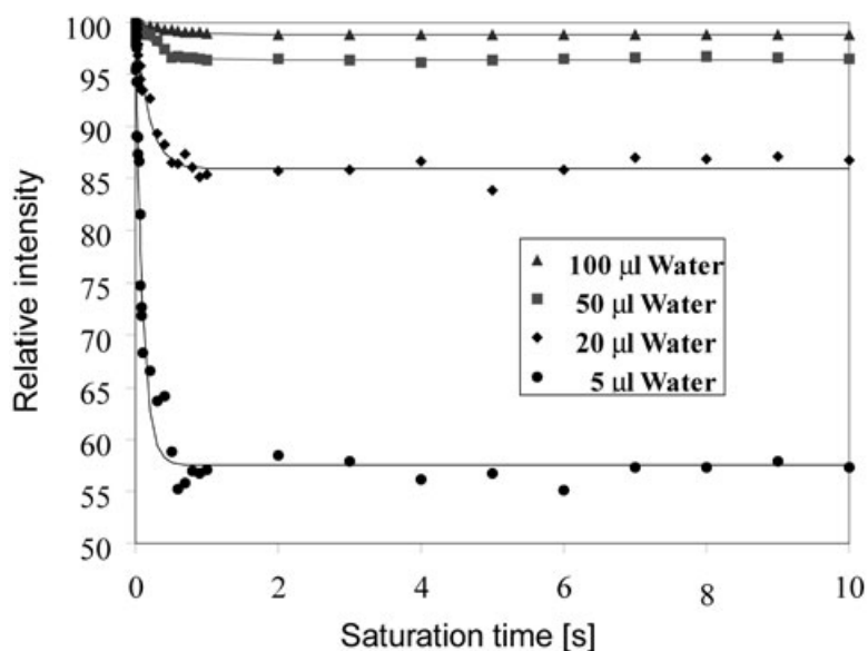
Fig. 3. ^1\text{H} -NMR Saturation-transfer experiments with [\text{Eu}(\mathbf{12})(\text{H}_2\text{O})](\text{CF}_3\text{SO}_3^-)_3 . To a soln of the complex (30 mg) in anhydrous \text{CD}_3\text{CN} (0.4 ml) were added 5, 20, 50, or 100 \mu\text{l} of \text{H}_2\text{O} . The saturation frequency was set to the bound \text{H}_2\text{O} resonance (55 ppm rel. to bulk \text{H}_2\text{O} at 0 ppm), with a B_1 value of 1200 Hz and different saturation duration times (0–10 s). The experiments were performed on a Varian Inova-500 spectrometer with a PFG/ID probe. The solid lines reflect the fits of the data to Eqn. 1 (see text) for a \tau_M value of 146 \pm 5 \mu\text{s} .
