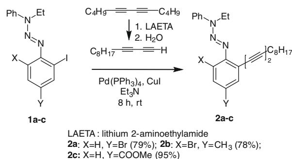
Scheme 1. Synthesis of ortho -(dodeca-1,3-diynyl)aryltriazenes via Pd/Cu-catalyzed cross-coupling of iodotriazenes with dodeca-1,3-diyne.
