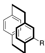
Figure 1. [2.2]Paracyclophane and sulfur derivatives.
