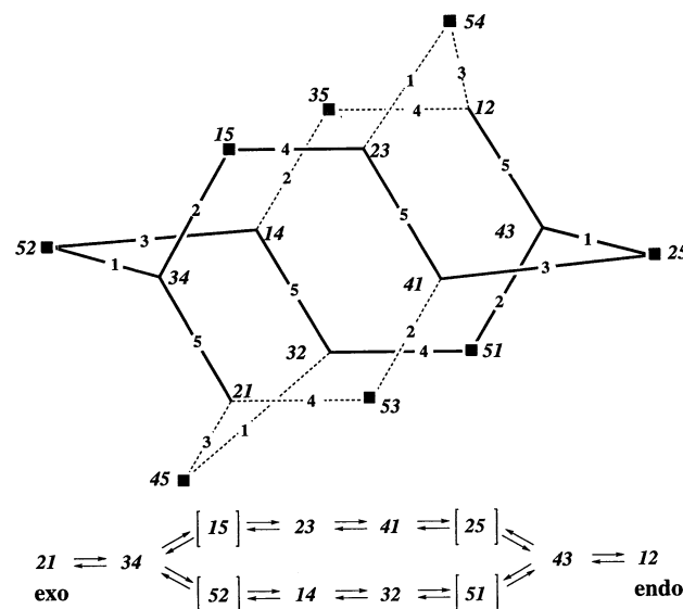
Fig. 4. Restricted Desargues–Levi diagram. The double digits correspond to diastereomers and the single digits to the pivot substituent of the pseudorotation process.
