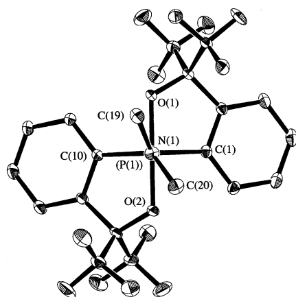
Fig. 6. ORTEP drawing of 7' (X = NMe 2 ) viewed along the direction of the axis of the P–N bond with thermal ellipsoids at 30% probability level. Hydrogen atoms have been omitted for clarity.
