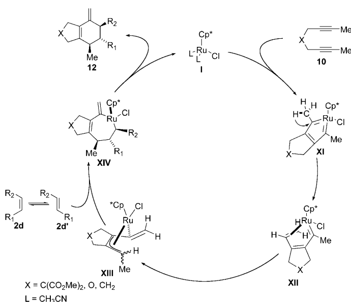
Scheme 9. New Ru II -catalyzed cycloisomerization of diyne 10 and conjugated alkenes 2 .
