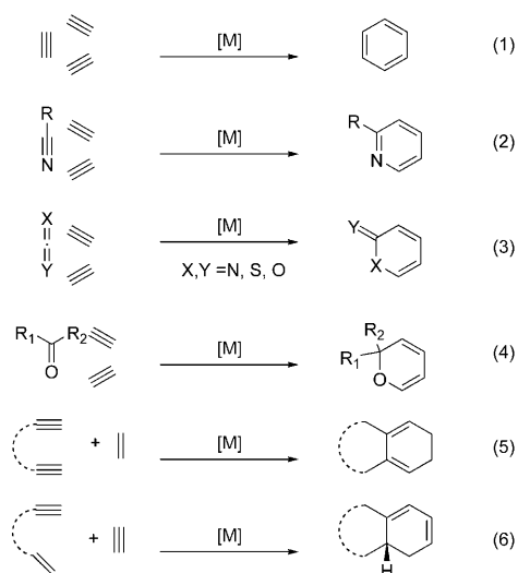
Scheme 1. Metal-catalyzed [2+2+2] cycloaddition reactions.
