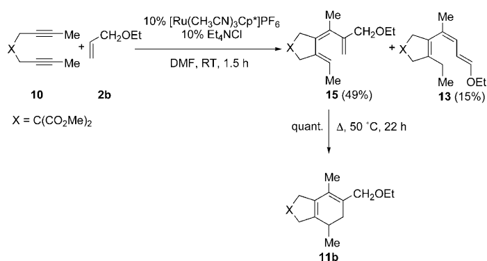
Scheme 7. "Formal" Ru-catalyzed [2+2+2] cycloaddition of disubstituted diyne 10 and ethyl allyl ether ( 2b ).
