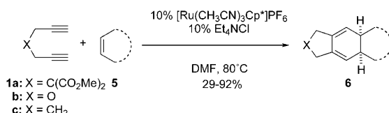
Scheme 3. Standard \text{Ru}^{\text{II}} -catalyzed [2+2+2] cycloaddition of 1,6-diynes 1 with cyclic alkenes 5 .
