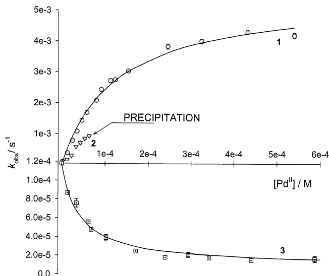
Fig. 2. Dependence of the observed pseudo-first-order rate constants for hydrolysis of 4 ( 2 \times 10^{-5} M) against concentrations of 1–3 at pH 8.0 (phosphate buffer, 25°C).
