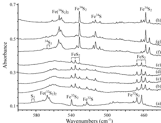
Figure 2. Infrared spectra in the 600\text{--}440\text{ cm}^{-1} region for products formed in the laser-ablated Fe reaction with discharged sulfur-34 enriched vapor during condensation in excess argon at 7 K: (a) normal ^{32}\text{S} isotopic sample deposited for 60 min, (b) 50/50 mixed ^{32,34}\text{S} isotopic sample, (c) after annealing to 30 K, (d) after annealing to 40 K, (e) after annealing to 48 K, (f) ^{34}\text{S} after sample deposition, (g) after annealing to 5 K, and (h) (c) after annealing to 43 K.
