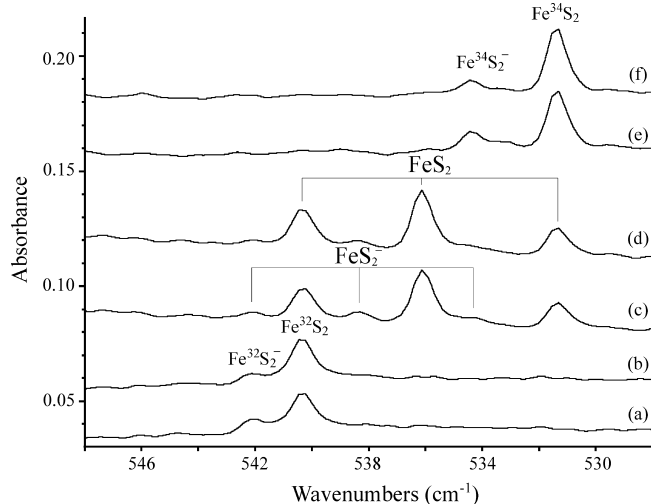
Figure 3. Infrared spectra in the 550\text{--}530\text{ cm}^{-1} region for products formed in the low-energy laser-ablated Fe reaction with discharged sulfur vapor during condensation in excess argon at 7 K: (a) normal ^{32}\text{S} isotopic sample deposited for 60 min, (b) after >220\text{ nm} irradiation, (c) 50/50 mixed ^{32,34}\text{S} isotopic sample, (d) after >220\text{ nm} irradiation, (e) ^{34}\text{S} after sample deposition, and (f) after >220\text{ nm} irradiation.
