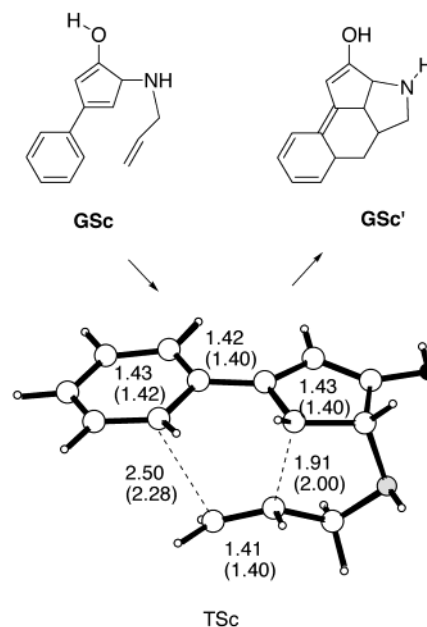
Figure 4. B3LYP/6-31G* transition structure for the model IMDA reaction (GSc \rightarrow TS \rightarrow GSc'). HF/6-31G* bond lengths (Å) are in parentheses.
