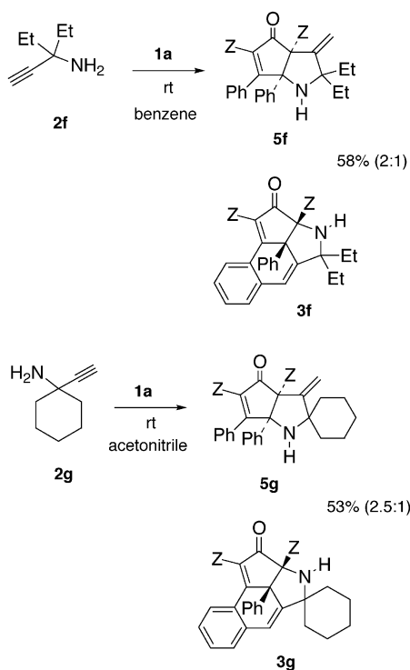
Scheme 5
