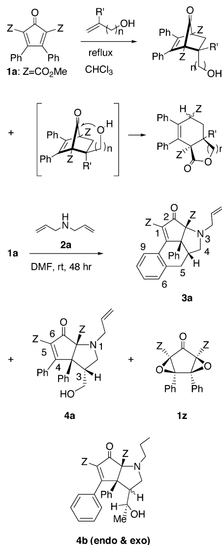
Scheme 1
