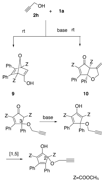
Scheme 10
