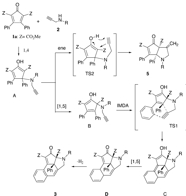
Scheme 7
