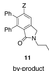
Scheme 4
