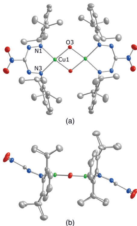
Figure 4. (a) Representation of the X-ray structure of (5)_2\text{Cu}_2(\text{OH})_2 with all non-H atoms shown as 50% thermal ellipsoids. (b) Alternate view by rotating part (a) by 90°. Selected interatomic distances (Å) and angles (deg): Cu1–O3, 1.9179(13); Cu1–O3', 1.9294(13); Cu1–N1, 1.9519(15); Cu1–N3, 1.9646(15); Cu1–Cu1', 3.0278(5); O3–Cu1', 1.9294(13); O3–Cu1–O3', 76.19(6); O3–Cu1–N1, 172.51(6); O3'–Cu1–N1, 96.95(6); O3–Cu1–N3, 98.50(6); O3'–Cu1–N3, 173.05(6); N1–Cu1–N3, 88.09(6); N3–Cu1–Cu1', 136.57(5); Cu1–O3–Cu1', 103.81(6).
