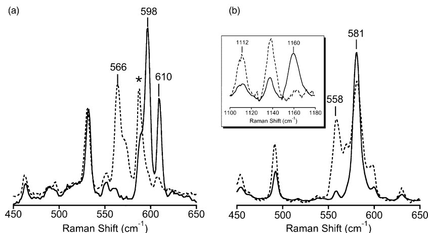
Figure 6. rR spectra of the frozen solutions resulting from oxygenations of (a) (4)Cu(CH 3 CN) (40 mM) and (b) (5)Cu(CH 3 CN) (10 mM) in THF at -80 °C, using 16 O 2 (solid line) or 18 O 2 (dashed line). The inset to plot (b) shows overtone bands. Excitation wavelengths were 457.9 and 514.5 nm, respectively. The asterisk indicates a solvent peak.
