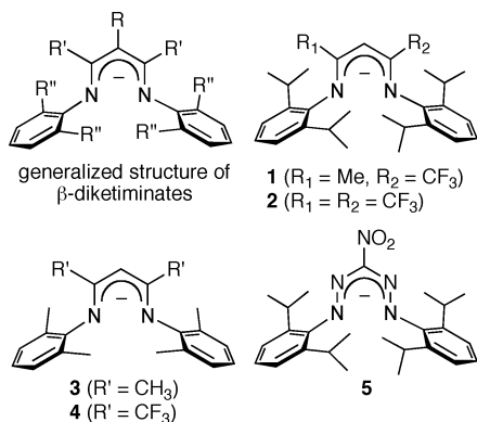
Figure 1. Diketiminate and formazan (5) ligands.
