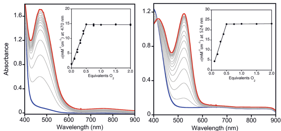
Figure 5. UV-vis changes accompanying oxygenation of (left) (4)Cu(CH 3 CN) and (right) (5)Cu(CH 3 CN) at -80 °C in THF, using starting concentrations of 0.2 or 0.1 mM, respectively. The initial and final spectra are in blue and red, respectively. The insets show the results of spectrophotometric titrations of the complexes with O 2 as linear fits to (left) data for two replicate runs or (right) average data from three replicate runs.
