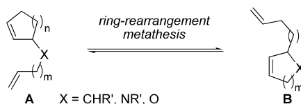
Scheme 1. Ring-Rearrangement Metathesis
