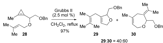
Scheme 7. RRM of a Cyclopropenylcarbonyl Prenyl Ether
