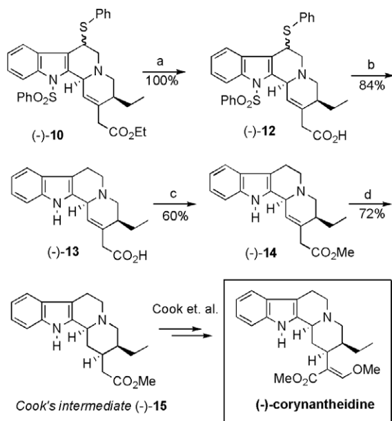
Scheme 3. Reagents and conditions: (a) \text{Ba}(\text{OH})_2 , \text{H}_2\text{O} , \text{THF}/\text{MeOH} (2:1), 50 °C, 30 min, 100%; (b) \text{Li} , \text{NH}_3 , \text{THF} , -78 °C then -33 °C, 84%; (c) thionyl chloride, \text{MeOH} , reflux, 1 h, 60%; (d) \text{H}_2 , \text{PtO}_2 , \text{MeOH} , rt, 30 min, 72%.
