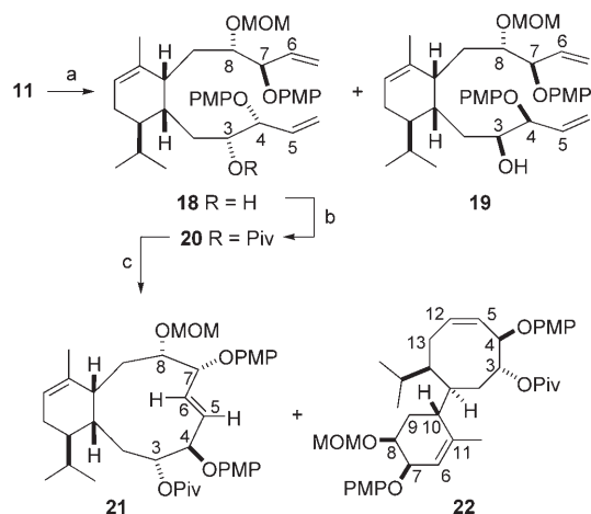
Scheme 4. Reagents and conditions: a) PMPOAllyl, sec -BuLi (1.4 M in cyclohexane), d IpcBOMe, BF 3 ·Et 2 O, THF, -78°C → 25°C, 40% 18 , 14% 19 ; b) PivCl, DMAP, DIPEA, CH 2 Cl 2 , 25°C, 83%; c) cat. 13 (30% mol), toluene, 110°C, 6.5 h, 27% 21 , 15% 22 . PMP= p -methoxyphenyl; Piv= tert -BuCO; DMAP=4-(dimethylamino)pyridine; DIPEA=diisopropylethylamine; Ipc=isopinocampheyl.
