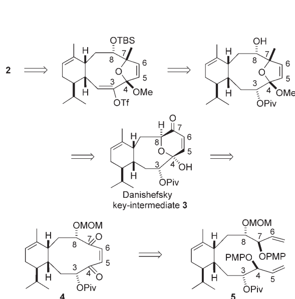
Scheme 1. Retrosynthetic analysis of eleutherobin ( 2 ).
