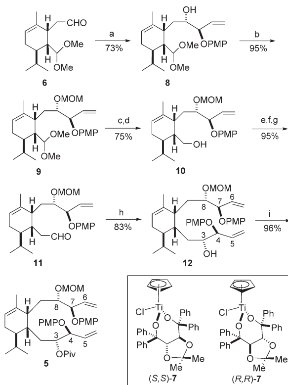
Scheme 2. Reagents and conditions: a) sec -BuLi (1.3 M in cyclohexane), PMPOAllyl, [TiCl(Cp)]{(S,S)-Taddol} ( 7 ), THF/Et 2 O (57:43), –78 °C → 0 °C, 73 %; b) DIPEA, TBAI, MOMCl, CH 2 Cl 2 , 25 °C, 95 %; c) LiBF 4 , CH 3 CN/H 2 O (98:2), 25 °C; d) NaBH 4 , EtOH, 25 °C, 75 % over two steps; e) MsCl, TEA, CH 2 Cl 2 , 0 °C → 25 °C, 95 %; f) KCN, [18]crown-6, CH 3 CN, 80 °C, quant.; g) DIBAL-H, toluene/hexane (1:2), –78 °C, quant.; h) sec -BuLi (1.4 M in cyclohexane), PMPOAllyl, [TiCl(Cp)]{(R,R)-Taddol} ( 7 ), Et 2 O/THF (81:19), –78 °C → 25 °C, 83 %; i) PivCl, DMAP, DIPEA, CH 2 Cl 2 , 25 °C, 96 %. PMP = p -methoxyphenyl; DIPEA = diisopropylethylamine; TBAI = tetrabutylammonium iodide; MOMCl = chloromethyl methyl ether; MsCl = methanesulfonyl chloride; TEA = triethylamine; DIBAL-H = diisobutylaluminum hydride; Piv = tert -BuCO; DMAP = 4-(dimethylamino)pyridine.
