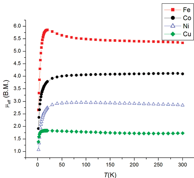
Figure 8. Plot of \mu_{\text{eff}} vs T for \text{MCl}_2\text{tripbipy} , \text{M} = \text{Fe}, \text{Co}, \text{Ni}, \text{Cu} .
