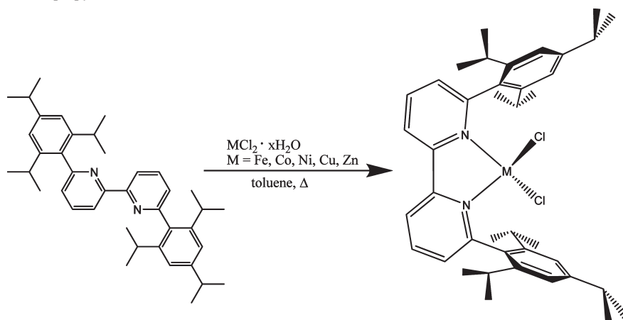
Scheme 2. Synthesis of MCl_2 tripbipy
