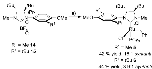
Scheme 3. Synthesis of new catalysts: reaction conditions: a) (CF 3 ) 2 CH 3 COK (1.5 equiv), PhMe then (PCy 3 ) 2 Cl 2 Ru=CHPh (1 equiv), 60 °C, 6 h. Only the major syn rotational isomer is shown above.
