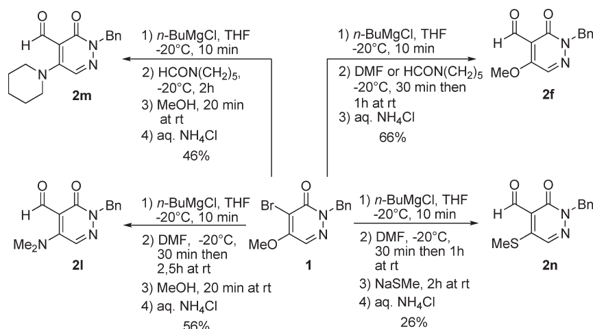
SCHEME 3. Plausible Mechanism Explaining the Different Reaction Products Obtained when a Workup with MeOH or aq \text{NH}_4\text{Cl} was Performed
