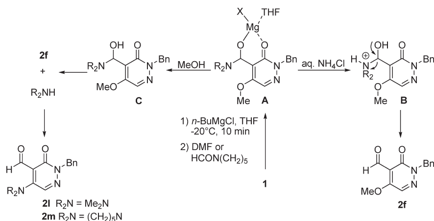
SCHEME 3. Plausible Mechanism Explaining the Different Reaction Products Obtained when a Workup with MeOH or aq \text{NH}_4\text{Cl} was Performed
