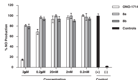
Figure 2. Effect of compounds 8a , 8b , and ONO-1714 on nitric production in primary peritoneal macrophages measured 48 h after activation.
