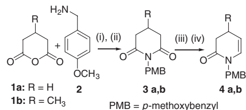
Scheme 1. Synthesis of olefins 4a and 4b . (i) THF, rt; (ii) Et 3 N, Ac 2 O (90–95% in two steps); (iii) DIBAL, CH 2 Cl 2 , –78 °C (80–85%); (iv) Et 3 N, MsCl, CH 2 Cl 2 , 0 °C (85–87%).
