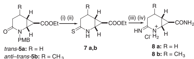
Scheme 2. Synthesis of amidines 8 . (i) TFA, 80 °C (20–25%); (ii) Lawesson's reagent (87–90%); (iii) MeOH sat. NH 3 ; (iv) HCl–MeOH (80–85%).
