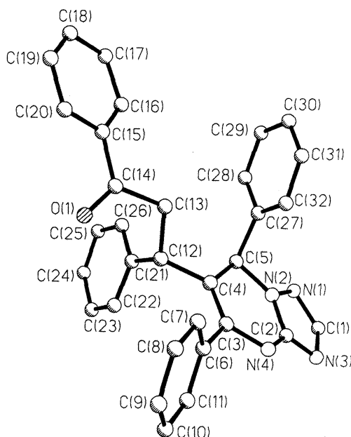
Figure 2. Perspective view of compound 3a .
