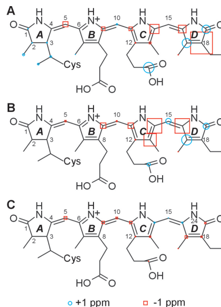
Figure 3. Changes in ^{13}\text{C} and ^{15}\text{N} chemical shift of the u- ^{13}\text{C} , ^{15}\text{N} -PCB chromophore in Cph1 \Delta 2 during the Pfr \rightarrow Lumi-F (A), Lumi-F \rightarrow Meta-F (B), and Meta-F \rightarrow Pr (C) transitions. For each transition, the starting state is taken as reference and the size of the circles and squares refers to the difference in ^{13}\text{C} and ^{15}\text{N} chemical shift in the next state.
