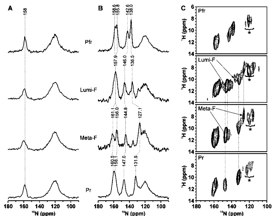
Figure 4. 1D ^{15}\text{N} spectrum of ^{15}\text{N}_{21} -PCB-Cph1 \Delta 2 (column A) and ^{15}\text{N} -PCB-Cph1 \Delta 2 (column B) in the Pfr, Lumi-F, Meta-F, and Pr recorded at 17.6 T with a spinning speed of 8 kHz and at 243, 173, 203, and 243 K, respectively. 2D ^1\text{H} - ^{15}\text{N} FSLG heteronuclear correlation spectra (column C) of Lumi-F and Meta-F were obtained from a Pfr:Pr (1:1) mixture.
