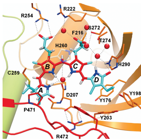
Figure 1. Chromophore binding pocket in Cph1 \Delta 2 phytochrome (pdb 2VEA).
