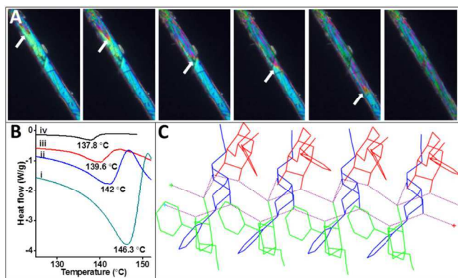
Figure 5. (A) Hot-stage polarizing microscopy images of polymorph \alpha showing the nucleation and growth. (B) DSC profiles of polymorph \alpha carried out at different heating rates 25 °C/min (i), 15 °C/min (ii), 10 °C/min (iii) and 5 °C/min (iv). (C) Crystal packing arrangement of an aged sample (kept at r.t. for 2 months) of polymorph \alpha .
