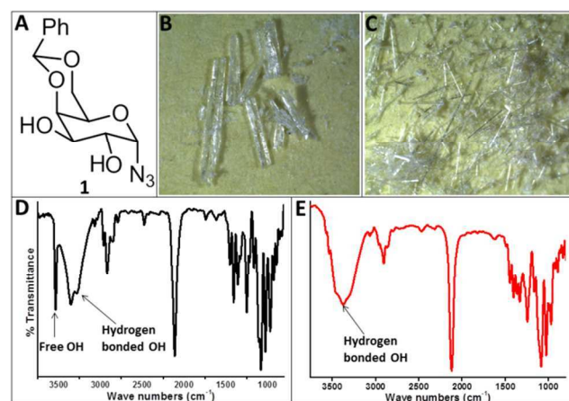
Figure 1. Chemical structure of compound 1 (A). Photograph of polymorphs, \alpha (B) and \beta (C). FTIR spectra of polymorphs \alpha (D) and \beta (E).
