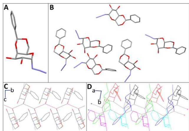
Figure 2. Asymmetric unit of polymorphs, \alpha (A) and \beta (B). Hydrogen atoms are omitted for clarity. Packing arrangement of \alpha viewed along 'a' direction (C) and \beta viewed along 'c' direction. Six conformers are color-coded as red, green, black, pink, cyan and blue (D).
