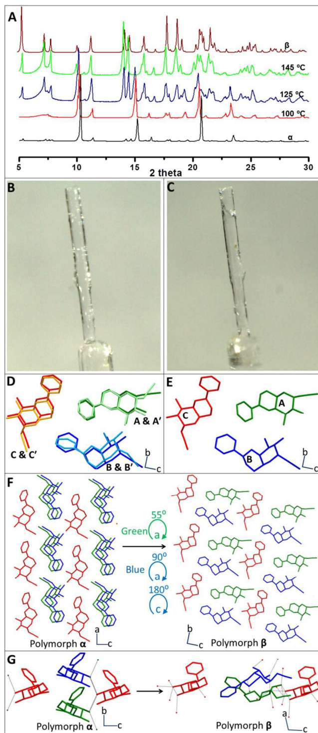
Figure 4. (A) Variable temperature PXRD patterns of polymorph \alpha . Photographs of single crystal of polymorph \alpha (B) before and (C) after heating at 140 °C for 5 minutes. (D) Two fold modulation of polymorph \beta viewed along the 'a' direction. (E) Three representative conformers of polymorph \beta in 'bc' plane. (F) Comparison of packing of polymorphs \alpha ('ac' plane) and \beta ('bc' plane). (G) Comparison of packing arrangements of polymorph \alpha ('bc' plane) with that of polymorph \beta ('ac' plane) showing the gain in number of hydrogen bonds after transition.
