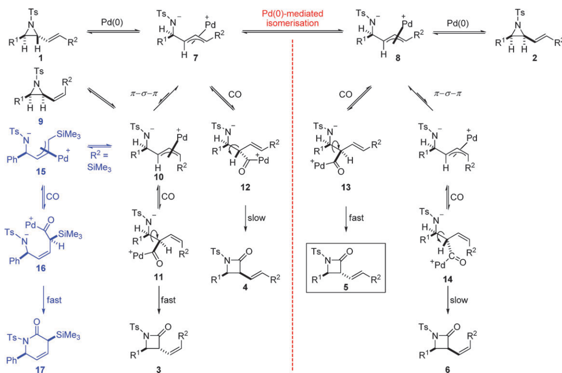
Scheme 2 Mechanism of conversion of vinyl aziridines into \beta - and \delta -lactams.
