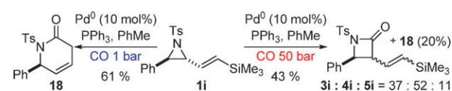
Scheme 3 Effect of pressure on the regioselectivity of carbonylation.
