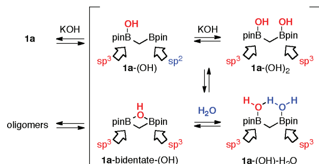
Figure 2. Possible borate intermediates.
