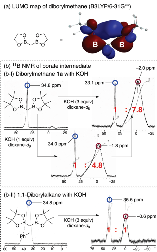
Figure 1. LUMO map and ^{11}\text{B} NMR spectra.
