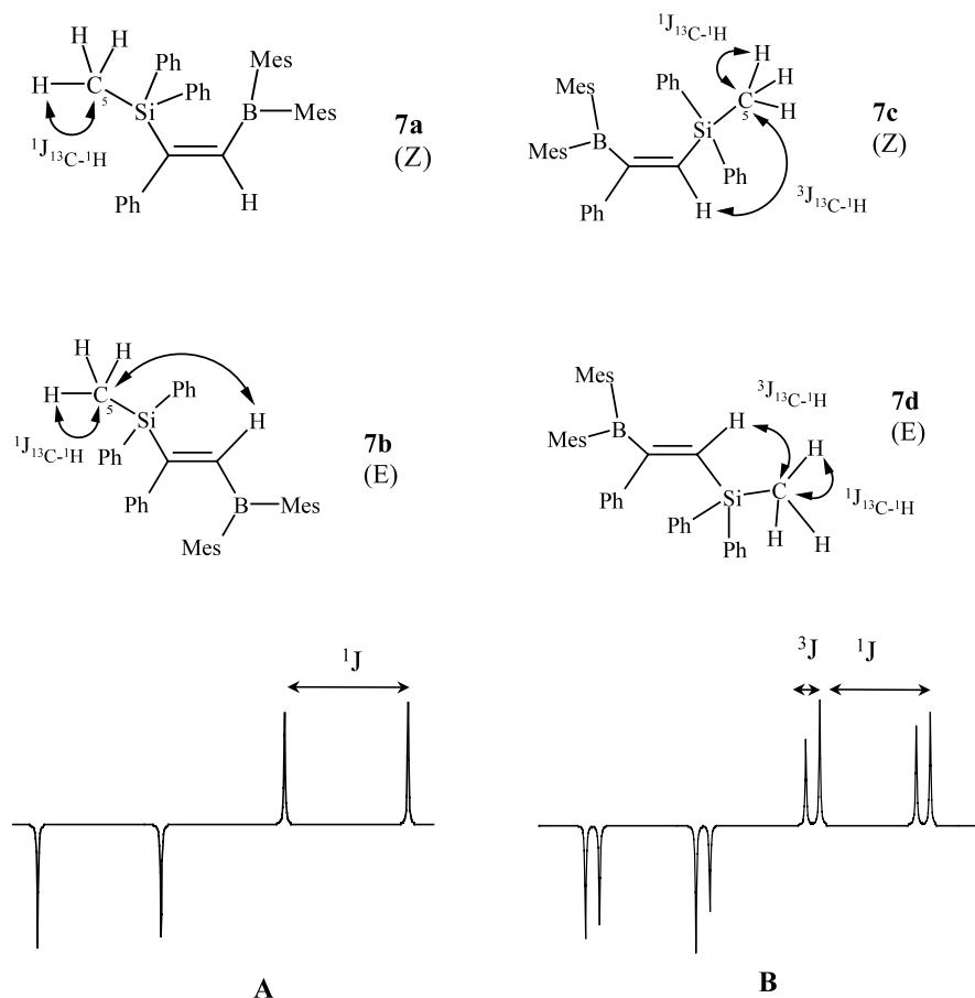
Scheme 2. Expected J_{13C-1H} coupling for C_5 related to Z/E isomers 7a–d and corresponding ^{13}C -NMR INEPT theoretical spectra.
