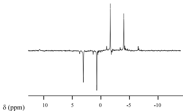
Fig. 1. Experimental ^{13}C -NMR INEPT spectrum of C_5 in product 7 .
