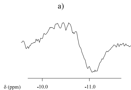
Experimental spectrum
