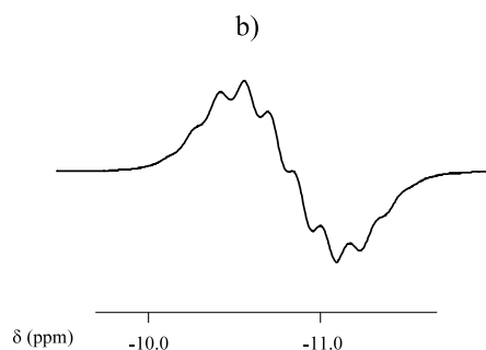
Simulated spectrum
