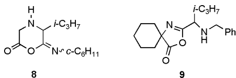
Figure 1. Previously isolated Ugi-4CC primary adducts.
