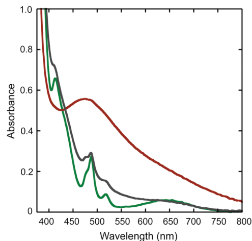
Figure 6. UV–vis spectra, recorded at 0 °C, of a reaction mixture of 8 (0.37 mM, green trace) in \text{CH}_3\text{CN}/\text{H}_2\text{O} (2:1), \text{NEt}_3 , and \text{H}_2\text{O}_2 to form a peroxo intermediate 8a (red trace). The gray trace corresponds to the product from the reaction.
