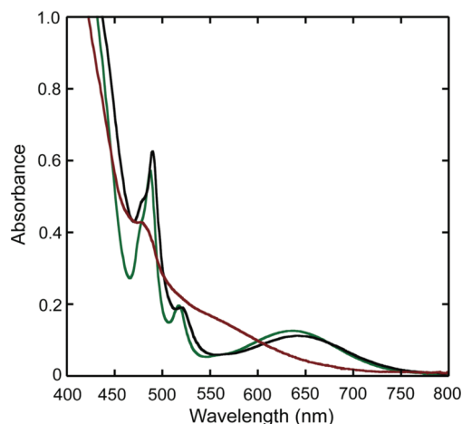
Figure 3. UV-vis absorption spectra of 1 mM solutions of 7 (black) and 8 (green) in \text{CH}_3\text{OH}/\text{CHCl}_3 (1:1) and of 6 (red) in \text{CH}_3\text{CN}/\text{H}_2\text{O} (10:1).
