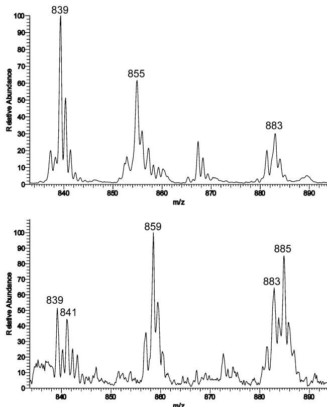
Figure 10. ESI mass spectrum of 7a at 295 K in CH 3 CN, displaying the isotope patterns for ions at m/z = 855 for \{[\text{Fe}_2(\mu\text{-O})(\mu\text{-}^{16}\text{O}_2)(\text{BPG}_2\text{DEV})] + \text{H}^+\} (top) and m/z = 859 for \{[\text{Fe}_2(\mu\text{-O})(\mu\text{-}^{18}\text{O}_2)(\text{BPG}_2\text{DEV})] + \text{H}^+\} (bottom). The peak m/z = 867 in the upper spectrum can be assigned to a formate-bridged diiron complex [\text{Fe}_2(\mu\text{-O})(\mu\text{-O}_2\text{CH})(\text{BPG}_2\text{DEV})]^+ , which is due to the presence of residual formic acid impurities.
