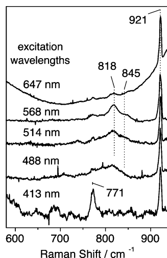
Figure 9. RR spectra of intermediate 6a obtained with different laser excitations at 110 K. All traces are normalized to the 921 cm⁻¹ solvent band.
