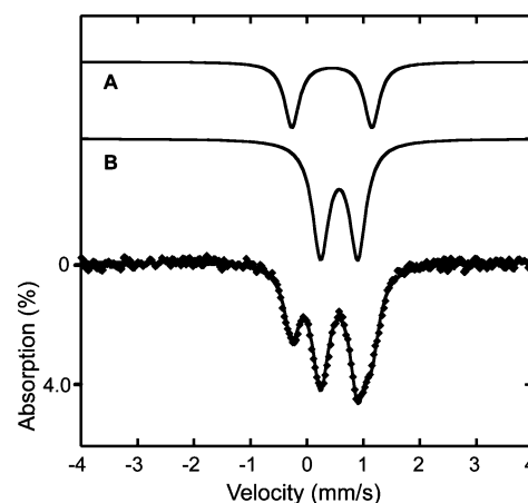
Figure 7. Zero-field Mössbauer spectrum [experimental data (◆)] recorded at 90 K for a frozen solution sample of the product of the reaction of 6 with excess \text{H}_2\text{O}_2 and a trace of \text{NEt}_3 . The sample contained 66% of 6a (B) and 34% of a diiron(III) species (A; \delta = 0.45 \text{ mm/s} and \Delta E_Q = 1.41 \text{ mm/s} ) with Mössbauer parameters similar to those of the starting material.
