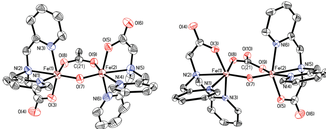
Figure 2. ORTEP diagram of 7 (left) and 8 (right) displaying thermal ellipsoids (50%). For clarity, the diethynylveratrole backbones, the \text{Ar}^{\text{iPrO}} group, and the \text{ClO}_4^- anion are not shown.
