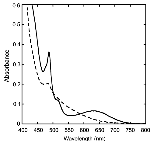
Figure 5. UV-vis spectra of 6 before (---) and after reaction with \text{CO}_2 (—) in a basic \text{CH}_3\text{OH}/\text{CH}_2\text{Cl}_2 (1:1) solution.
