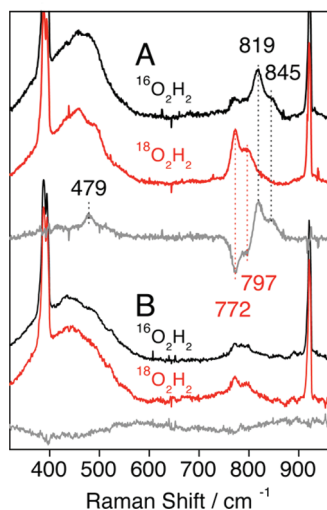
Figure 8. RR spectra of intermediate 6a (A) and its decomposition product (B) obtained with 568-nm excitation at 110 K. Sharp Raman bands below 400 and above 900 cm⁻¹ correspond to solvent vibrations.
