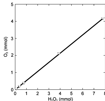
Figure 11. O 2 formation from 0.078 to 7.8 mmol of H 2 O 2 at 0 °C catalyzed by 8 (2 mL of 0.4 mM solution in CH 3 CN/H 2 O, 2:1) and 10 \mu\text{L} of NEt 3 .
