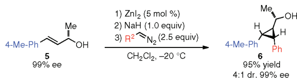
Scheme 5. \text{ZnI}_2 -Catalyzed Simmons–Smith Cyclopropanation
