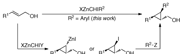
Scheme 1. Synthesis of 1,2,3-Substituted Cyclopropanes Using Zinc Carbenoids
