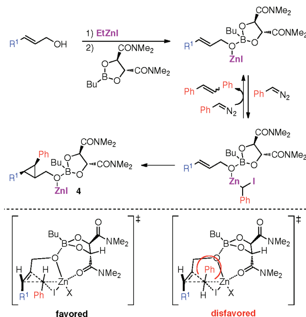
Scheme 3. Proposed Mechanism
