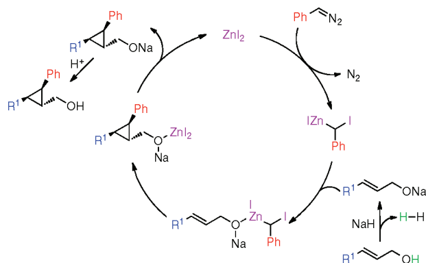
Scheme 4. Catalytic Cycle of the \text{ZnI}_2 -Catalyzed Simmons–Smith Cyclopropanation
