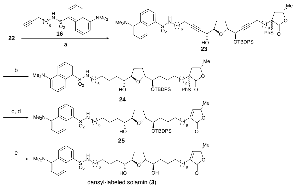
Scheme 6. Reagents and Conditions: (a) 16 , Zn(OTf) 2 , i -Pr 2 NEt, (1 R ,2 S )- N -methylephedrine, toluene, rt, 66% (91:9 dr); (b) H 2 (3 atm), (Ph 3 P) 3 RhCl, benzene, rt, 73%; (c) m CPBA, CH 2 Cl 2 , 0 °C; (d) toluene, reflux, 68% in two steps; (e) 48% HF aq., MeCN, rt, 71%.
