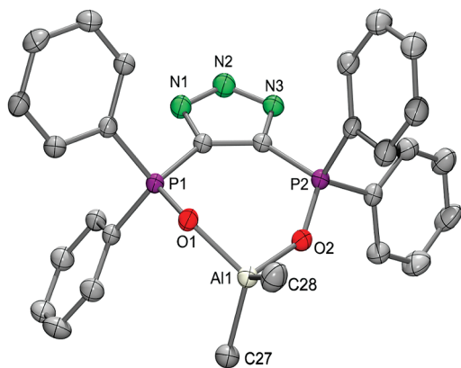
Figure 2. Perspective view of 4a (triclinic) with thermal ellipsoids at 50% probability. All hydrogen atoms are omitted for clarity.
