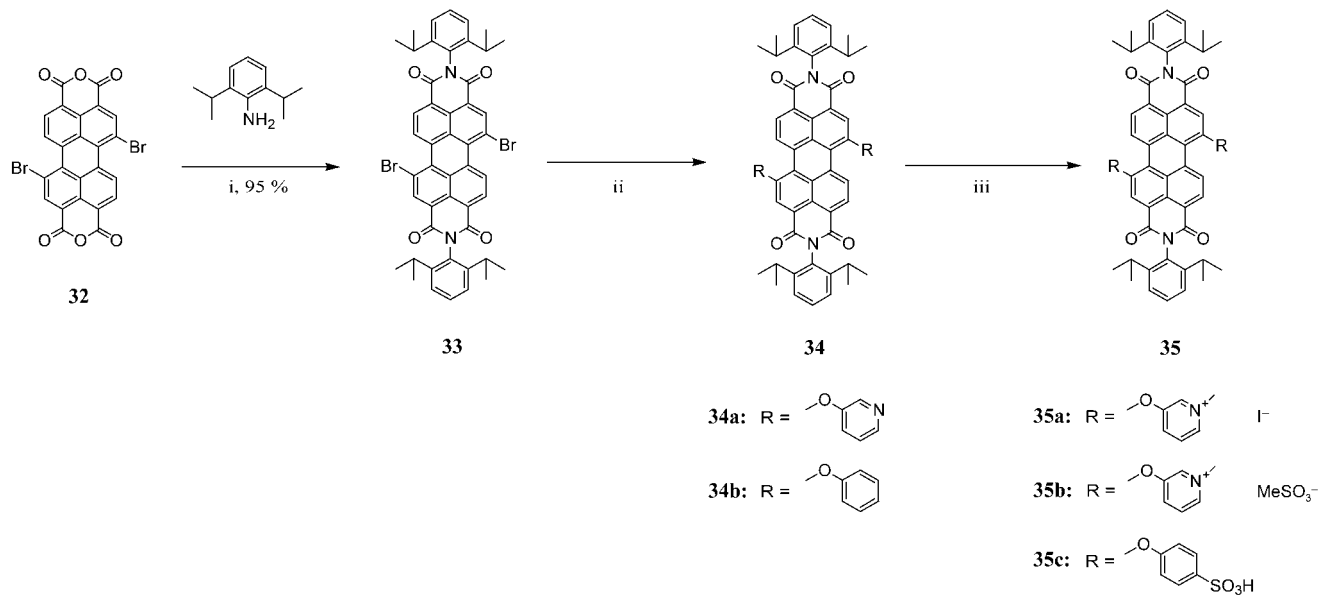
Scheme 6. i) 2,6-Diisopropylaniline, propionic acid, 140 °C, 5 h, 95 %; ii) a: compound 33 , 3-pyridinol ( 15 ), NMP, K 2 CO 3 , 80 °C, 15 h, 81 %; b: compound 33 , phenol, NMP, K 2 CO 3 , 80 °C, 15 h, 80 %; iii) a: compound 34a , methyl iodide, chloroform, reflux, 24 h, b: compound 34a , methyl iodide, methanol, reflux, 24 h, 94 %; silver methanesulfonate, methanol, RT, 5 h, 90 %; c: compound 34b , conc. sulfuric acid, RT, 15 h, 94 %.
