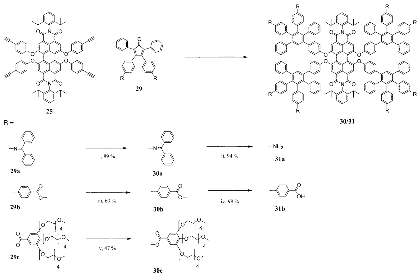
Scheme 5. i) Compound 29a , o -xylene, 20 h, 170 °C, 89 %; ii) compound 30a , THF, HCl (5 M), 94 %; iii) compound 29b , o -xylene, diphenyl ether, 40 h, 175 °C, 60 %; iv) compound 30b , THF, KOH, H 2 O, 42 h, 80 °C, 98 %; v) compound 29c , o -xylene, 24 h, 170 °C, 47 %.
