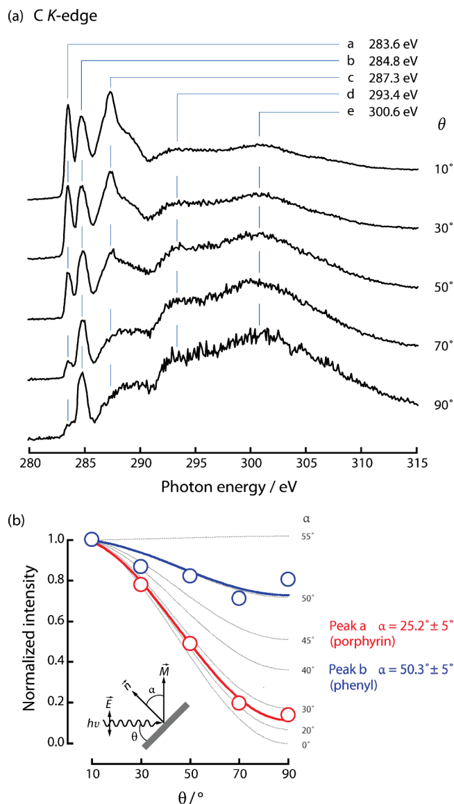
Figure 6. (a) C K-edge NEXAFS spectra acquired at five angles of photon incidence ( \theta ) for a \sim 0.5 ML coverage of [SAC]P–Mn(III)Cl on Ag(100). (b) Curve fitting analysis of the photon angle dependence of \pi^* resonances a and b to determine the corresponding macrocycle and phenyl tilt angles ( \alpha ) respectively.
