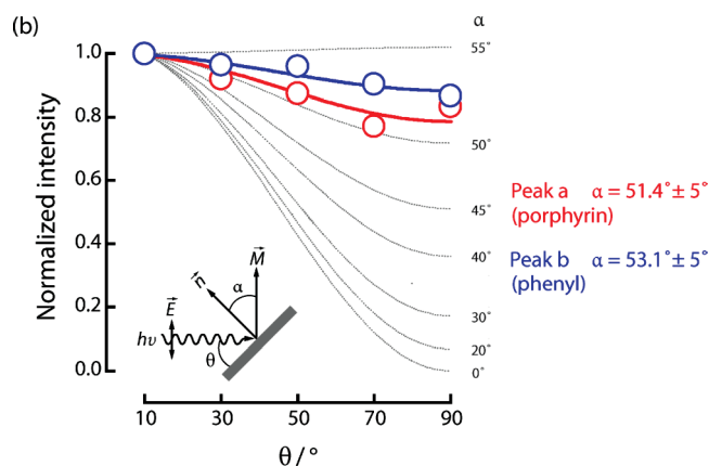
Figure 11. (a) C K-edge NEXAFS spectra acquired at five angles of photon incidence \theta for a \sim 1 ML coverage of the one-legged porphyrin [SAC]P–Mn(III)Cl on Ag(100). (b) Curve fitting analysis of the angle dependence of \pi^* resonances a and b to determine the corresponding \pi -system tilt angles \alpha .
