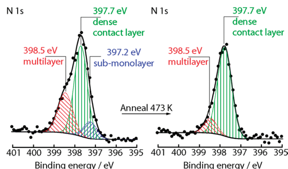
Figure 8. N 1s XP spectra for a high coverage of porphyrin as deposited (left) and after annealing to 473 K (right).
