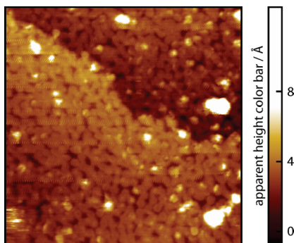
Figure 9. STM image ( 300 \times 300 \text{ Å}^2 , V_{\text{tip}} = 1.21 \text{ V} , I = 0.84 \text{ nA} ) of the densely packed contact layer of the one-legged porphyrin acquired after multilayer deposition and annealing to 473 K. White blobs are molecules in the second layer, as judged by apparent height.
