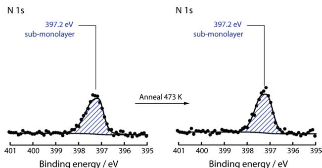
Figure 2. N 1s XP spectra of a low (submonolayer) dose of one-legged porphyrin acquired before (left) and after annealing to 473 K (right) for 15 min.
