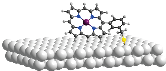
Figure 12. Proposed adsorption geometry of the one-legged porphyrin in the dense contact layer tethered to Ag(100). Macrocycle and phenyl tilt angles with respect to the surface are \sim 50^\circ and \sim 53^\circ respectively.
