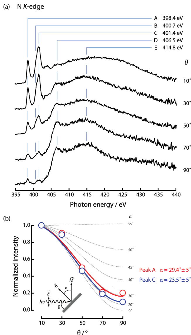
Figure 4. (a) N K-edge NEXAFS spectra acquired at five angles of photon incidence ( \theta ) for a \sim 0.5 ML coverage of [SAC]P–Mn(III)Cl on Ag(100). (b) Curve-fitting analysis of the photon angle dependence of \pi^* resonances A and C to estimate the corresponding macrocycle tilt angle, \alpha .
