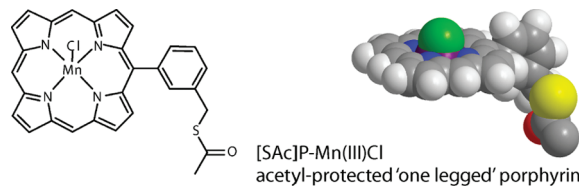
Figure 1. Molecular structure and 3D space-filling model for the “one-legged” porphyrin, [SAc]P–Mn(III)Cl.
