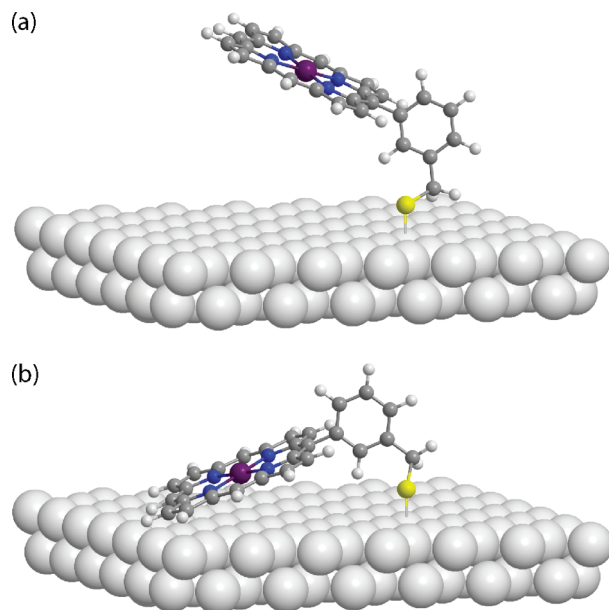
Figure 5. Two possible orientations of the one-legged porphyrin tethered to Ag(100) corresponding to the same macrocycle tilt angle of \sim 25^\circ – 30^\circ : (a) porphyrin tilted upward and (b) porphyrin tilted downward.
