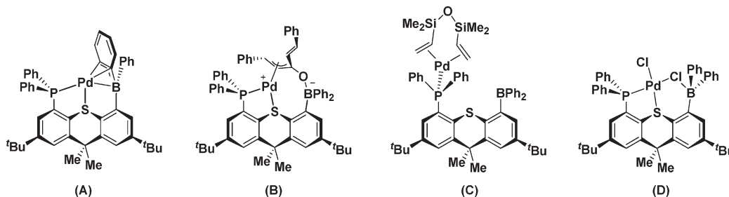
Figure 1. Examples of different metal-TXPB bonding modes: (A) Triarylborane \eta^3 -BCC-coordination. (B) Zwitterionic boratoxyallyl complex formation induced through binding of an enone co-ligand (dba). (C) TXPB \eta^1 -P-coordination induced by metal–diene coordination. (D) Chloride occupying a bridging position between the metal and the borane.
