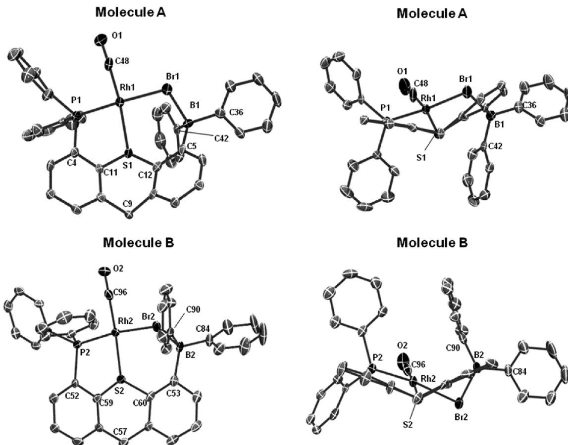
Figure 4. Solid-state structure of [\text{RhBr}(\text{CO})(\text{TXPB})]\cdot\text{hexane (2)}\cdot\text{hexane} with ellipsoids at 50% probability. tert -Butyl and \text{CMe}_2 methyl groups, hydrogen atoms, and solvent are omitted for clarity.
