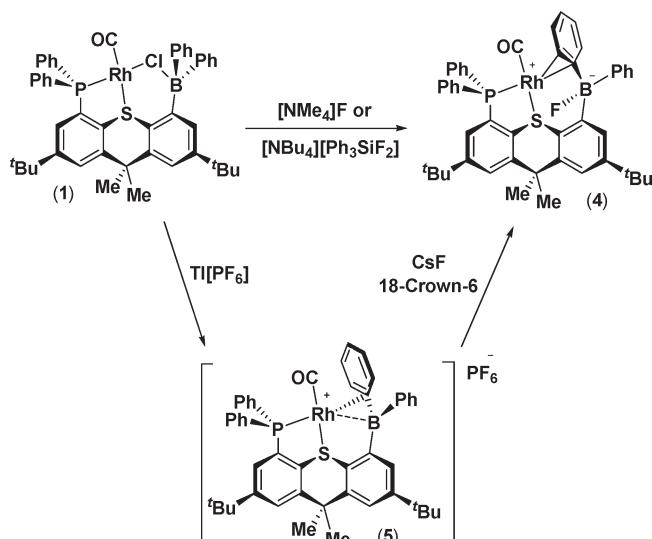
Scheme 2. Preparation of Complexes 4 and 5
