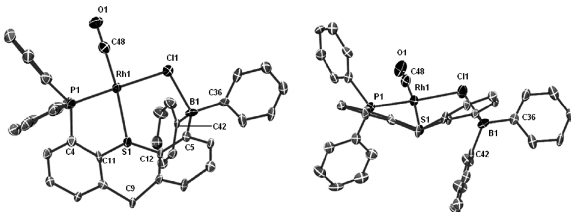
Figure 3. Solid-state structure of [\text{RhCl}(\text{CO})(\text{TXPB})] \cdot \text{hexane} (1) \cdot \text{hexane} with ellipsoids at 50% probability. tert -Butyl and \text{CMe}_2 methyl groups, hydrogen atoms, and solvent are omitted for clarity.
