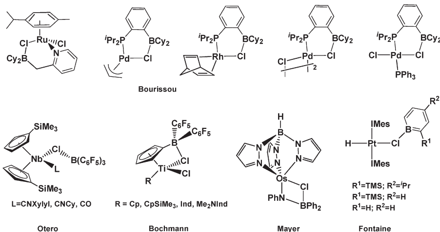
Figure 2. Complexes exhibiting a metal–halide–borane bridging interaction, not including TXPB complexes. Xyl = 2,6-dimethylphenyl; \text{C}_9\text{H}_6\text{NMe}_2 = 2-(dimethylamino)indenyl; IMes = 1,3-di(2,4,6-trimethylphenyl)imidazolin-2-ylidene.
