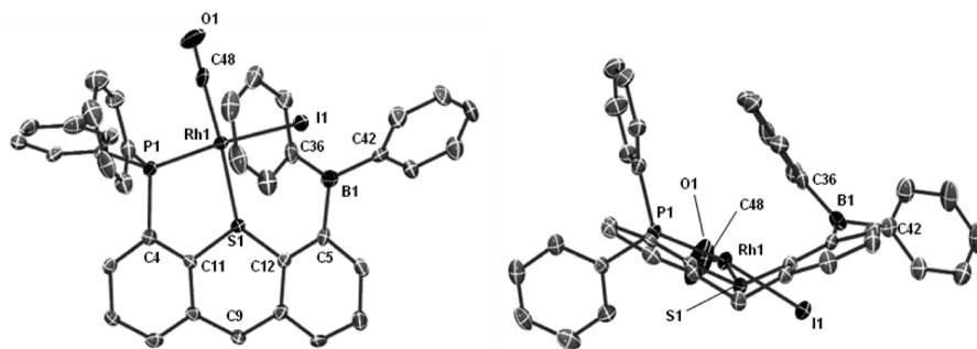
Figure 5. Solid-state structure of [\text{RhI}(\text{CO})(\text{TXPB})] \cdot \text{hexane} ( 3 )·hexane with ellipsoids at the 50% probability level. tert -Butyl and \text{CMe}_2 methyl groups, hydrogen atoms, and solvent are omitted for clarity.
